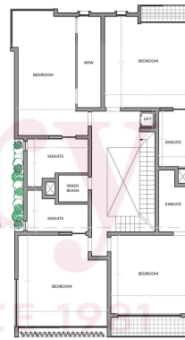
PROPOSED FIRST FLOOR scale 1:100
