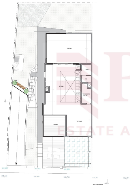
PROPOSED GROUND FLOOR scale 1:100
