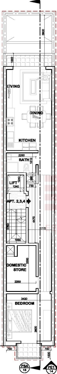
PP3 12 PROPOSED FIRST, SECOND & THIRD FLOOR SCALE 1:100
