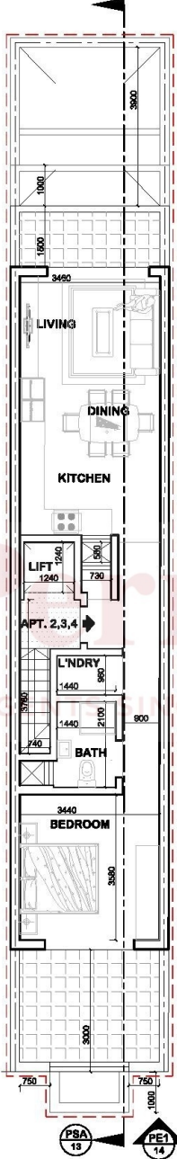
PP4 12 PROPOSED RECESSED FLOOR SCALE 1:100
