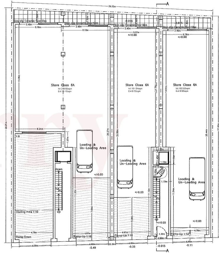
Ground Floor Level Proposed Scale 1:100
