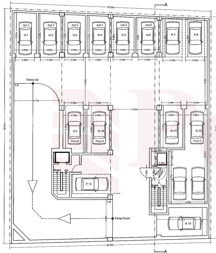
Basement Level -1 Proposed Scale 1:100 Build-Up Area - 717.24 sqm Number of Garages / Parking Spaces - 14
