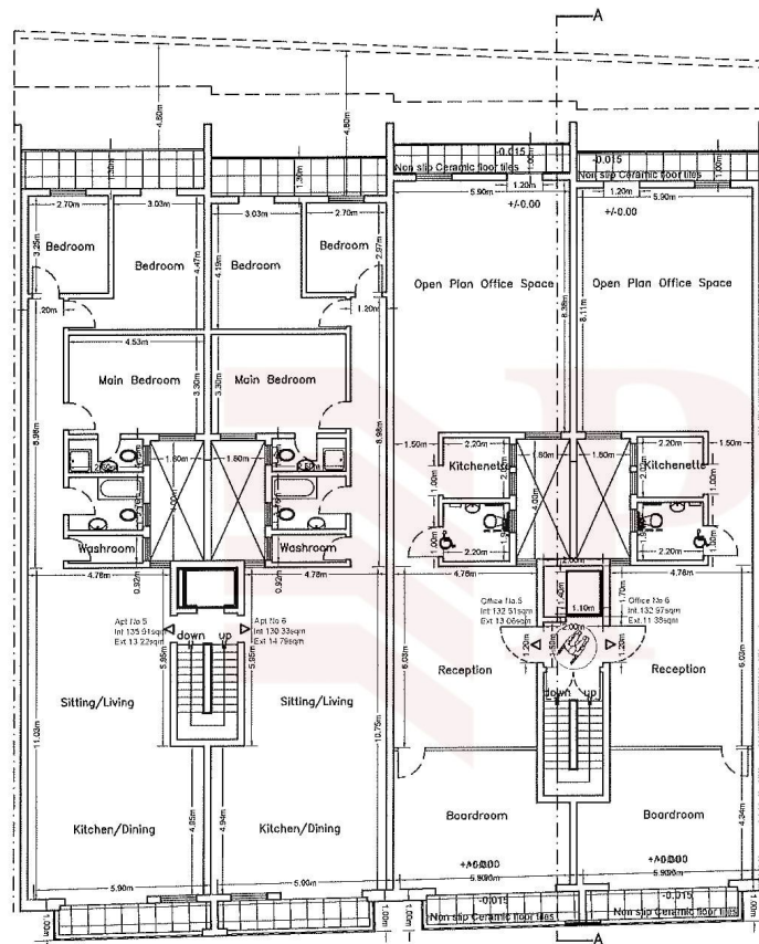
Third Floor Levels Proposed Scale 1:100
