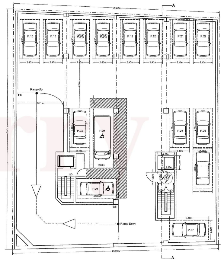
Basement Level -2 Proposed Scale 1:100 Built-Up Area - 717.24 sqm Number of Garages /Parking Spaces - 14
