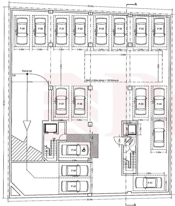
Basement Level -3 Proposed Scale 1:100 Built-Up Area - 717.24 sqm Number of Garages /Parking Spaces - 16
