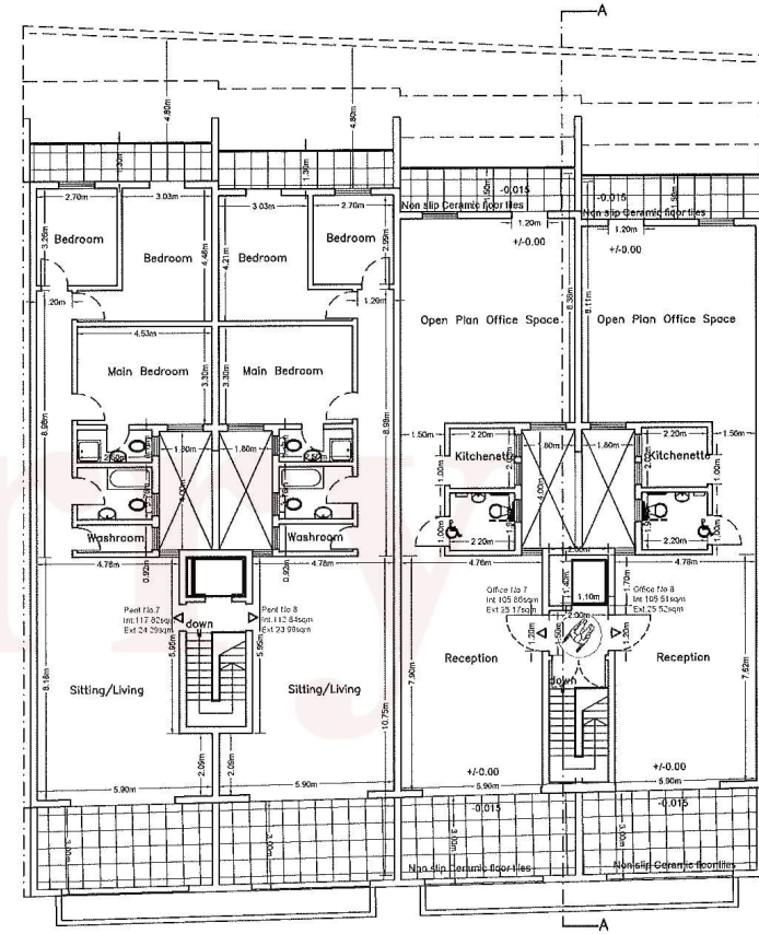
Setback Floor Level Proposed Scale 1:100
