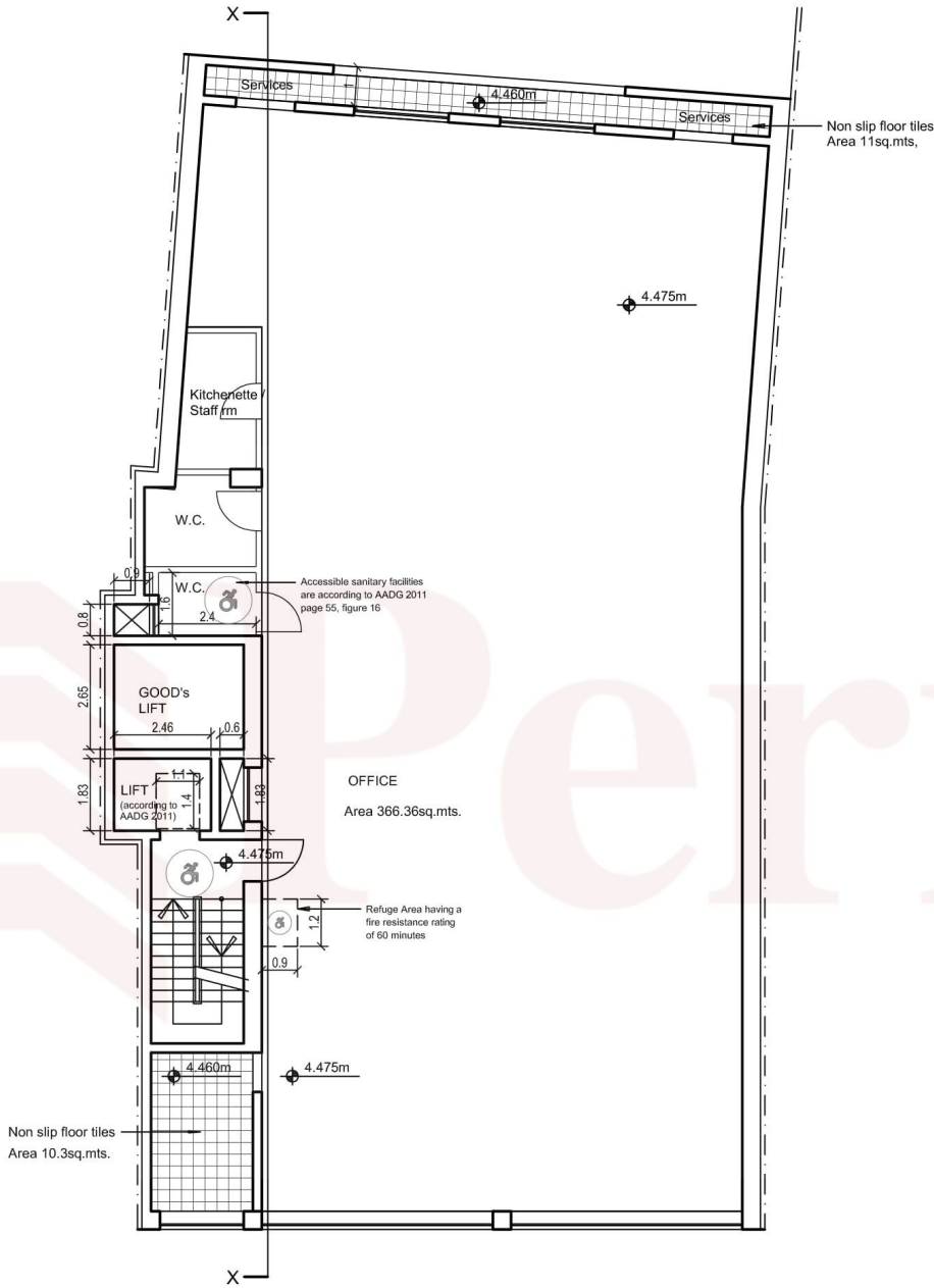
FIRST FLOOR PLAN Built up Area = 447.50sq.m.
