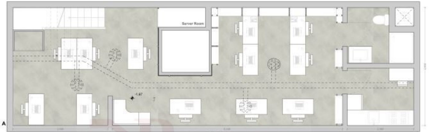
Proposed Basement Level scale 1:50
