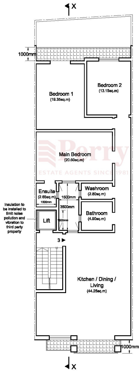
Approved Third Floor Level Scale 1:100
