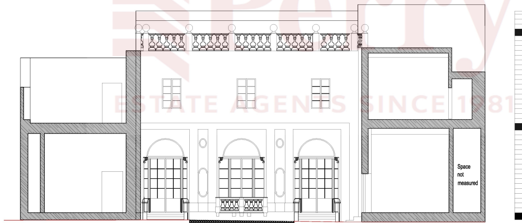
Back Sectional Elevation C - View from Garden Scale 1:50
